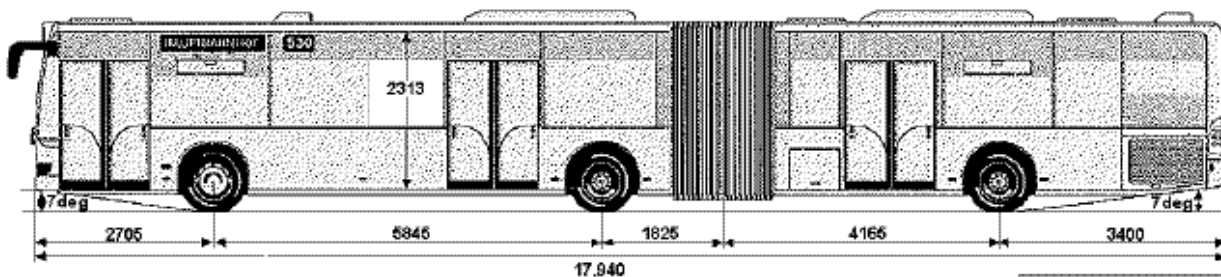
Citaro G, 3-door
